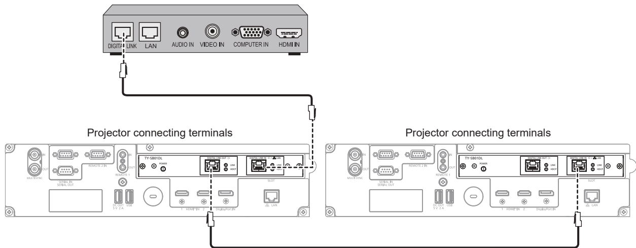
Example of twisted-pair-cable transmitter
