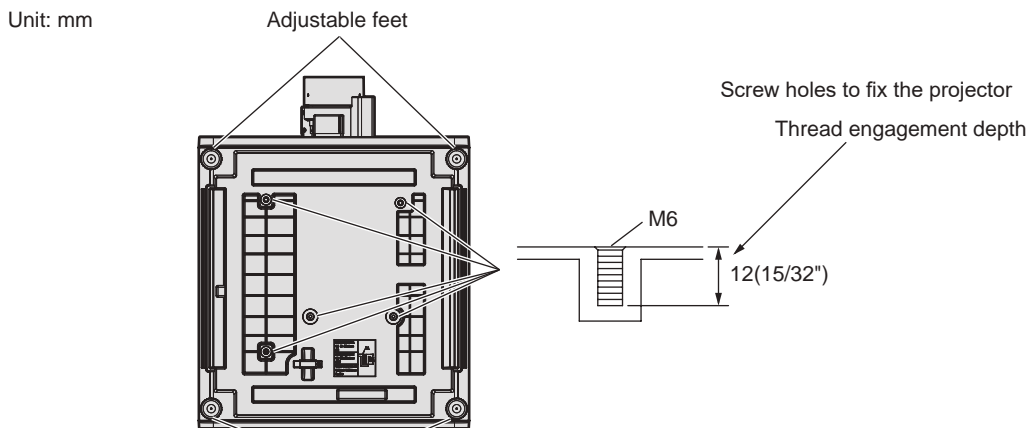
Adjustable feet Positions of screw holes to fix projector and adjustable feet
