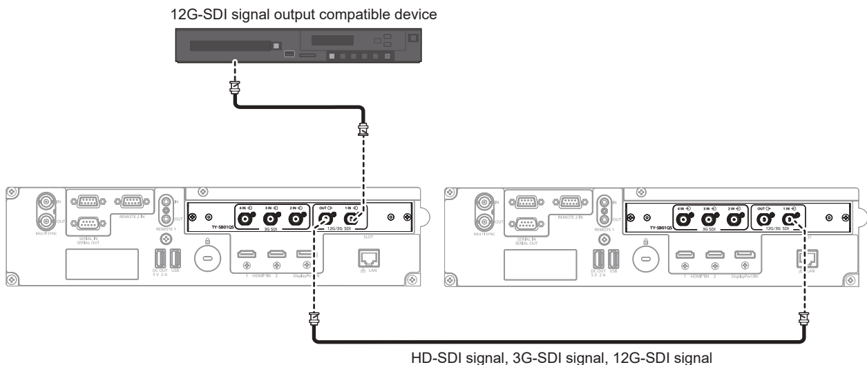
HD-SDI signal, 3G-SDI signal, 12G-SDI signal
