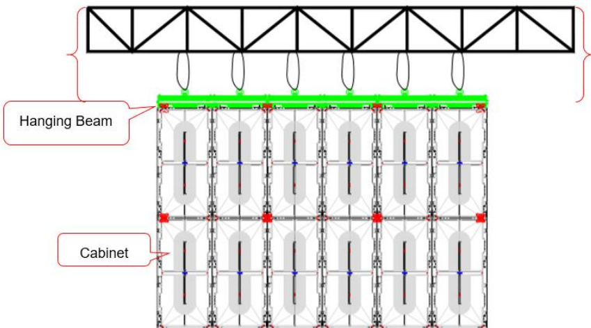
Figure 2-10 Installation of Hanged Cabinets (3)2.3 Wiring for LED Display
