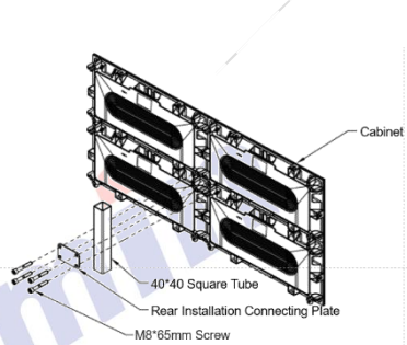
Figure 2-7 Rear Installation Details
