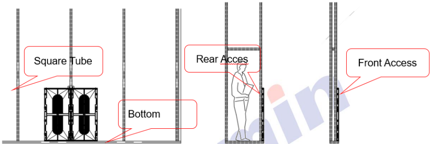
Figure 2-2 Cabinet Fastening
