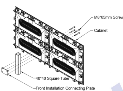
Figure 2-6 Front Installation Details
