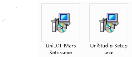
Fig 3-2 Software Installation
