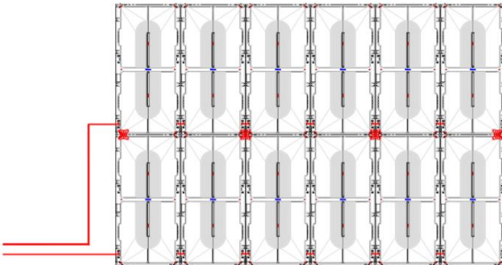
Figure 2-13 Power Cable Connection Diagram
