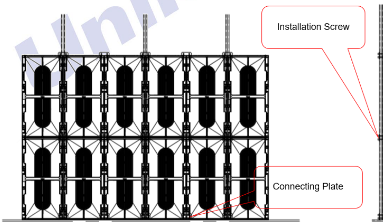
Figure 2-3 Rear View of Cabinet Installation
