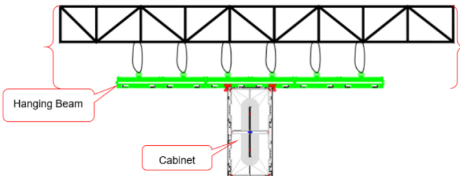
Figure 2-8 Installation of Hanged Cabinets (1)
