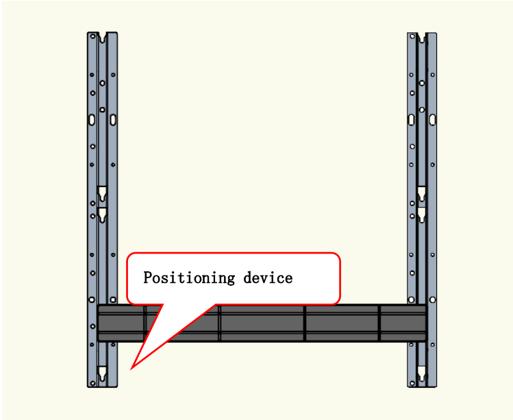
Fig. 2-18 Mounting the back strip according to the positioning device
