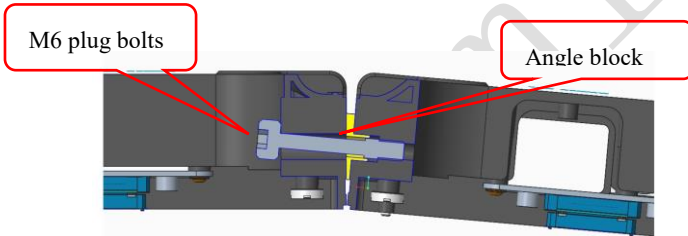
Fig 2-28 Internal drawing of left and right cabinet splicing
