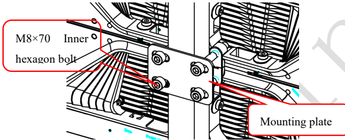
Fig 2-8 Back view of front maintenance Installation Details
