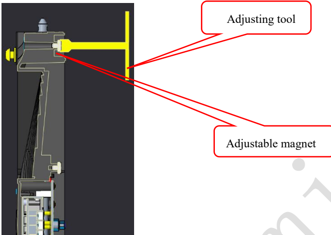
Fig 2-34 Schematic diagram of module flatness adjustment
