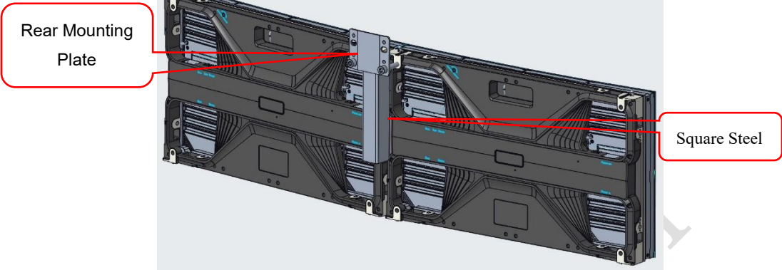
Fig 2-35 Splicing finish of left and right cabinet
