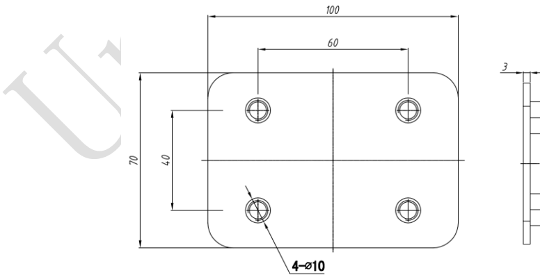
Fig 2-6 Front Connecting Plate
