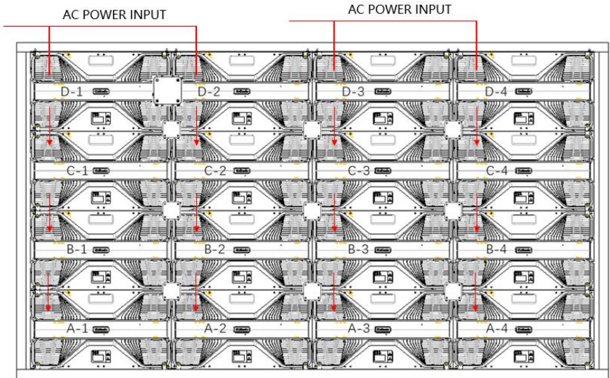
Fig 2-36 Power Cable Connection Diagram of ULWIII1.2
