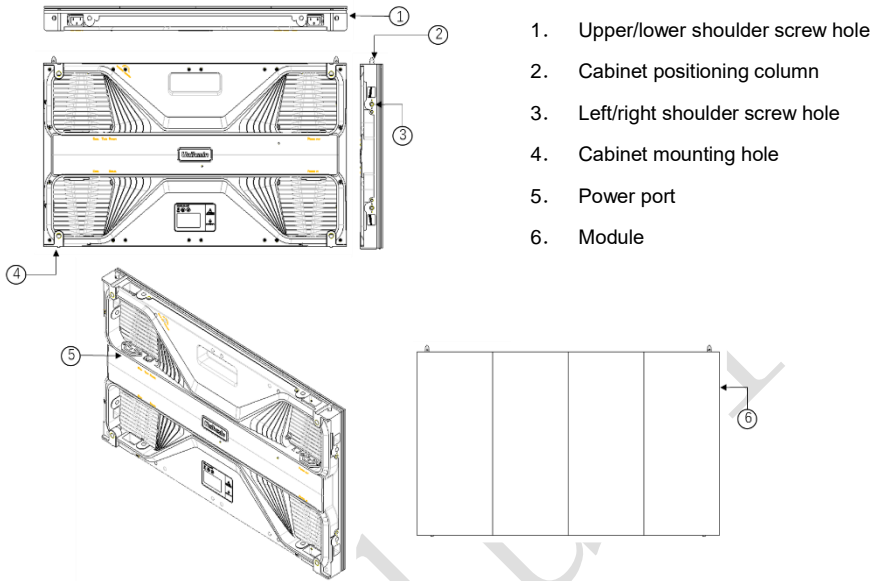
Fig 1-1 Cabinet Appearance
