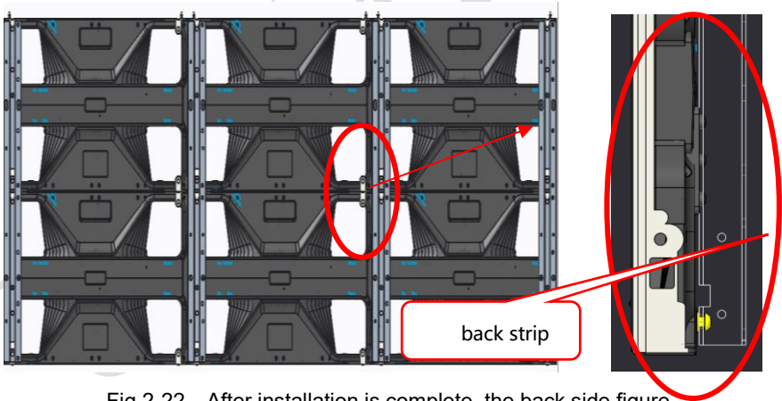
Fig 2-22 After installation is complete, the back side figure
