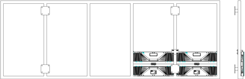
Fig 2-10 Cabinet Fastening
