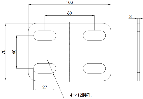
Fig 2-13 Rear maintenance installation plate
