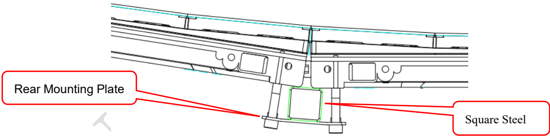
Fig 2-34 Internal drawing of left and right cabinet splicing
