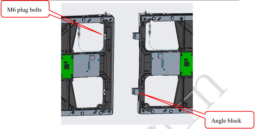
Fig 2-33 Splicing of left and right cabinet
