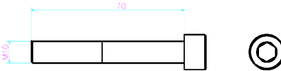
Fig 2-14 Rear installation M10×70 Inner hexagon bolt
