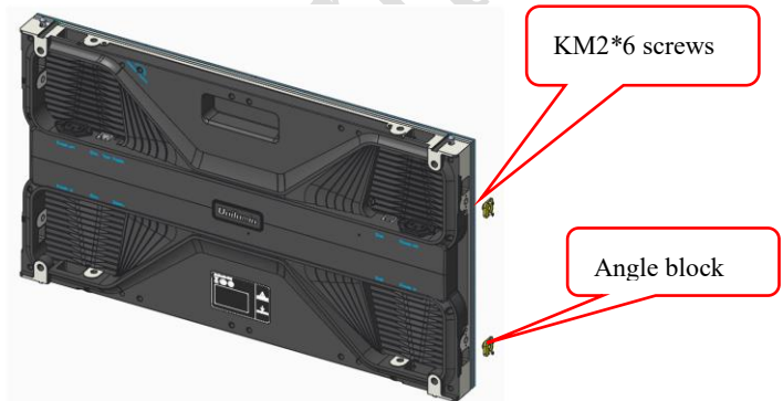
Fig 2-25 Installing angle block 1
