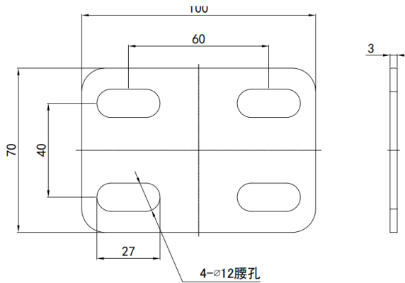
Fig 2-30 Rear Mounting Plate
