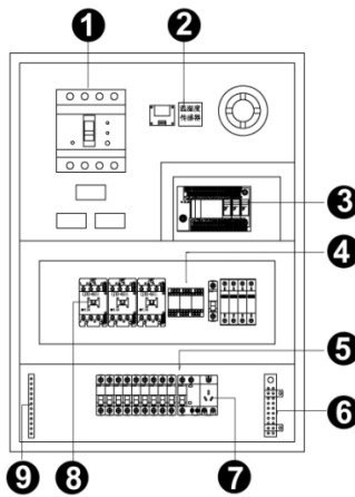
Fig 2-37 Internal Structure of Distribution Box
