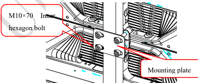
Fig 2-15 Back view of rear maintenance Installation Details
