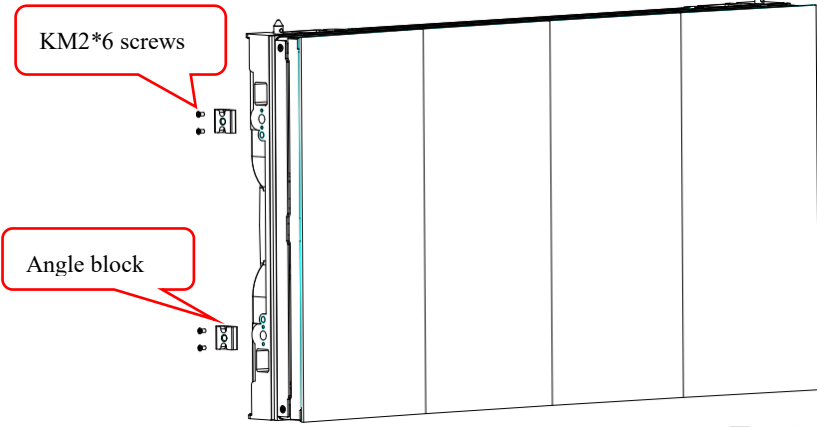
Fig 2-31 Installing angle block 1
