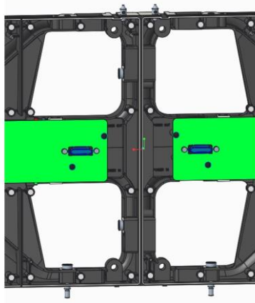
Fig 2-29 Splicing of left and right cabinets completed
