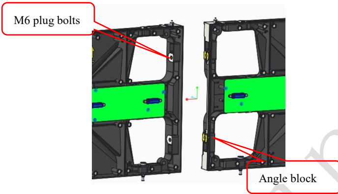
Fig 2-27 Splicing of left and right cabinet
