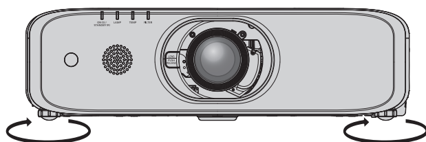
Maximum adjustable range Adjustable feet: 23 mm (29/32") each
